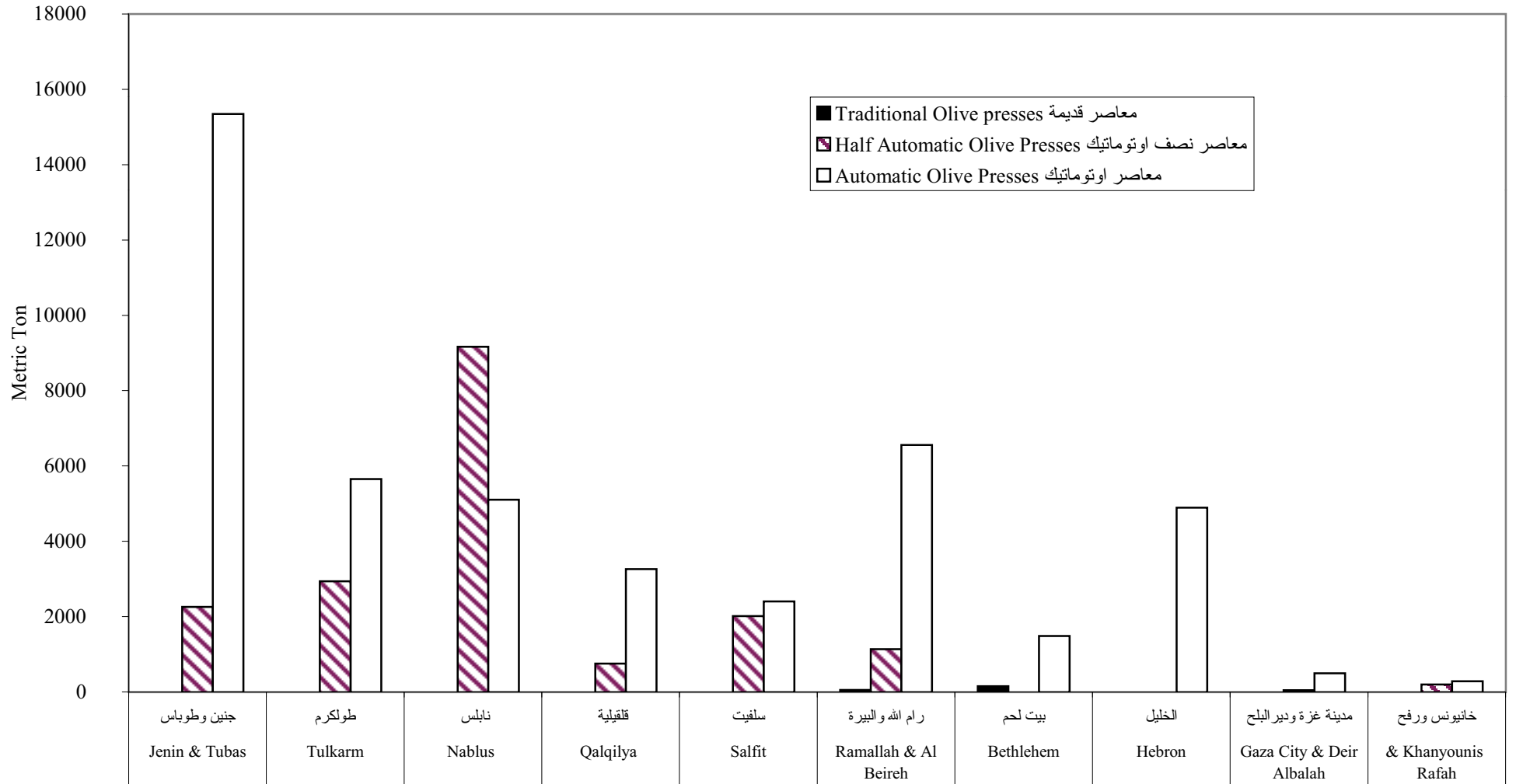
Figure 2: Quantity of Olive Pressed by Automation Level and Governorate, 1998
